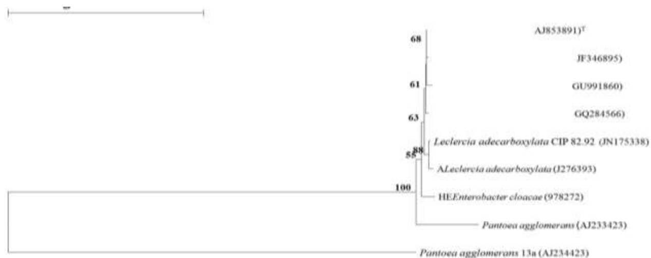
Figure 1: Phylogenetic trees based on comparative analysis of 16S rRNA gene sequences showing the relationship of the representative strain 13a among the family Enterobacteriaceae. The gene bank/ accession numbers of the sequence are given in parentheses.
